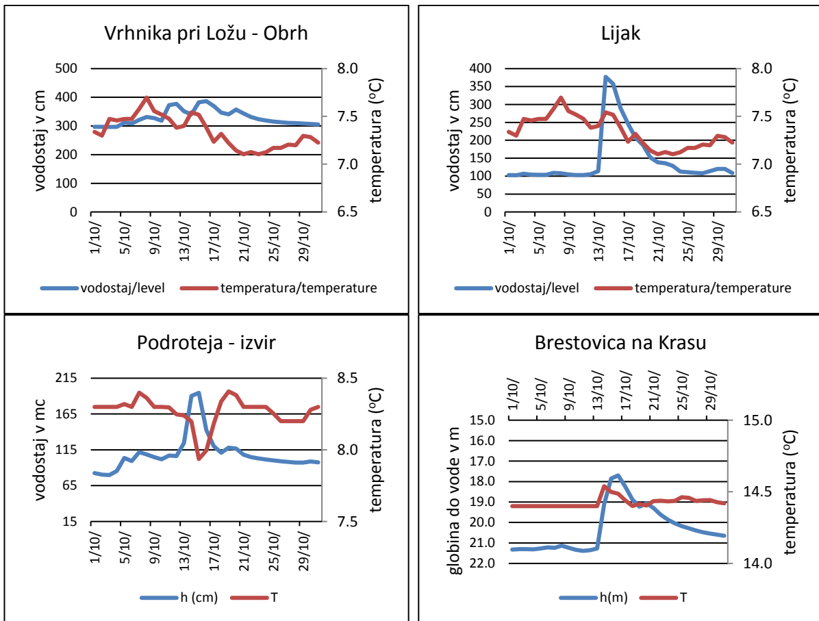
Slika 2. Grafi dnevne gibanja vodostajev in temperature na izbranih lokacijah kraških vodonosnikov. Figure 2. Daily water levels and temperatures on selected locations of karstic aquifers.
