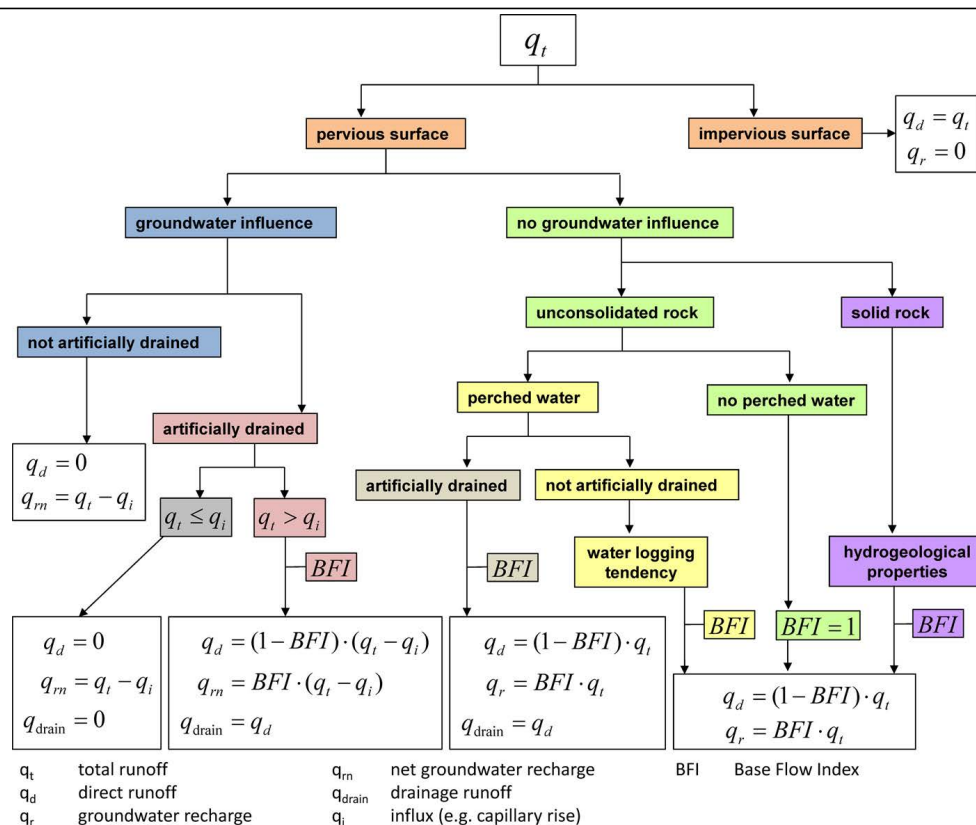
Figure 2-5: Site characteristics that determine groundwater recharge in GROWA.
