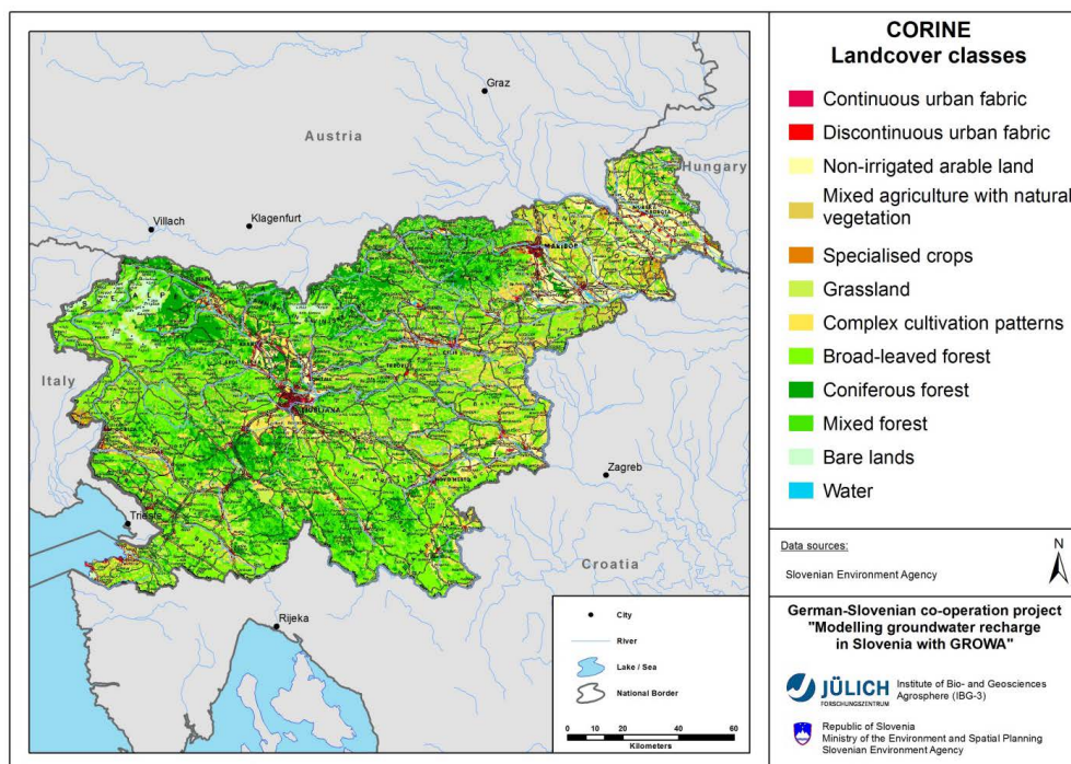
Figure 3-7: The CORINE Landcover units in Slovenia (CLC, 2000).
