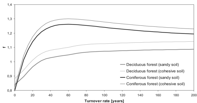
Figure 2-3: Long-term means of the parameter for deciduous (broad-leaved) and coniferous forests and different soil types depending on the turnover rate.
