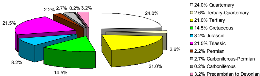
Figure 3-15: Frequency distribution by area of the most important stratigraphic units in Slovenia.
