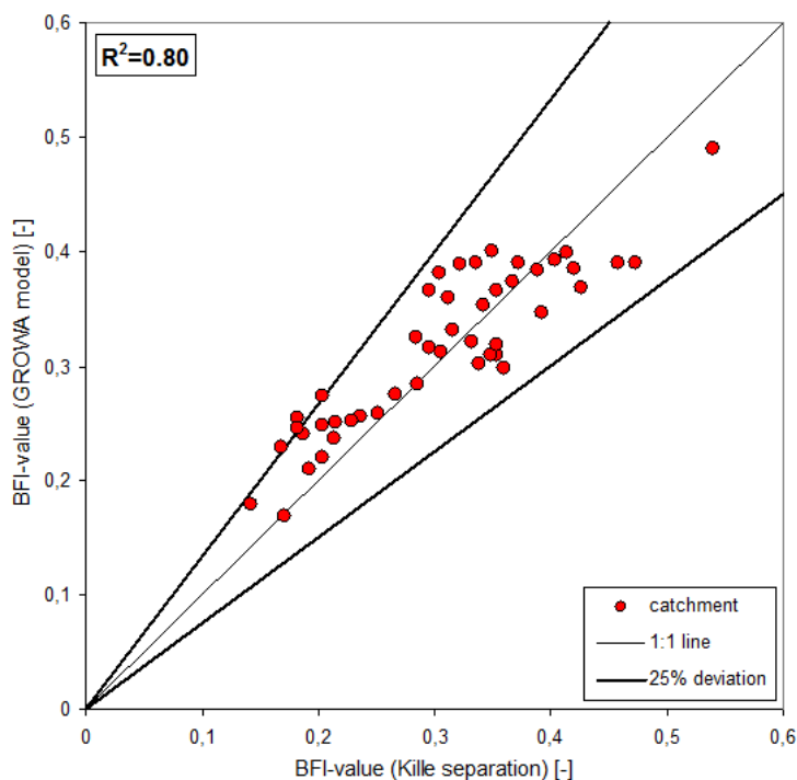
Figure 4-6: Comparison of measured and calculated BFI-values for the 46 catchment areas in Slovenia used for BFI calibration.
