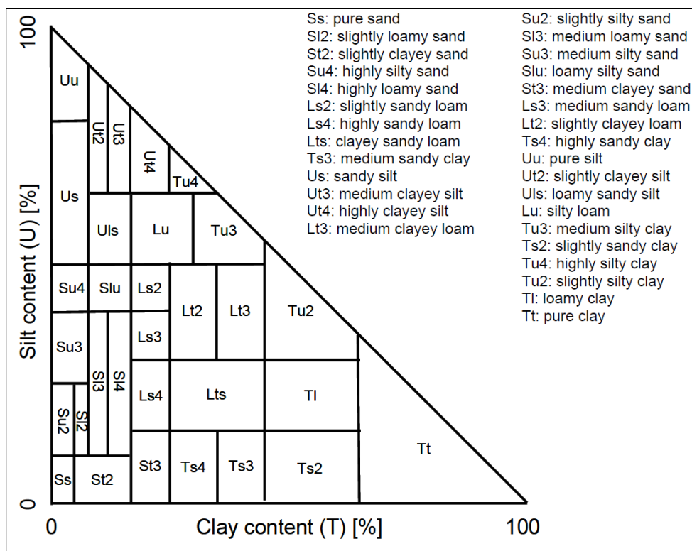
Figure 3-10: Definition of the German soil texture classes according to Ad-hoc-AG Boden (2005).
