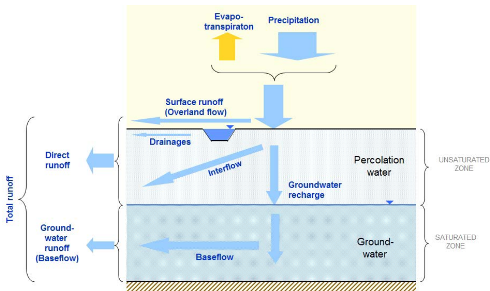
Figure 2-1: Water balance components considered in GROWA model (adapted from Wendland et al., 2010).
