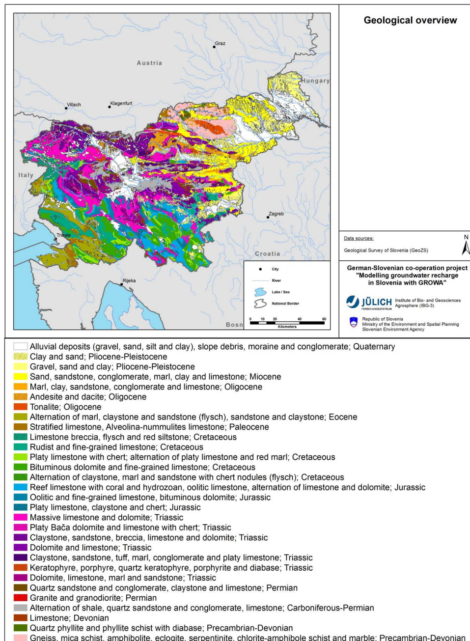
Figure 3-14: Geological overview of Slovenia, compiled from basic geological map of SFRJ 1:100,000 (OGK1, 1967-1998) and basic geological map of Slovenia 1:250,000 (Buser, 2010).
