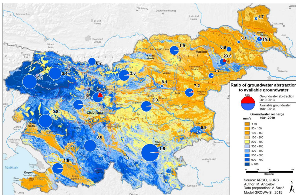
Figure 7-5: Ratio of groundwater abstraction (2010-2013) to mean long term available groundwater (1981-2010) by groundwater bodies, together with groundwater recharge by GROWA-SI (Uhan et al., 2015b).
