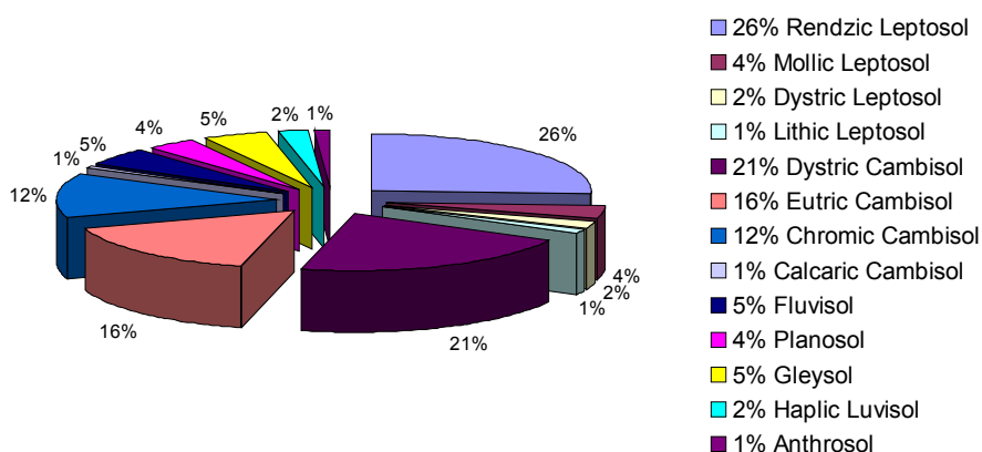
Figure 3-9: Frequency distribution of the main soil types in Slovenia.
