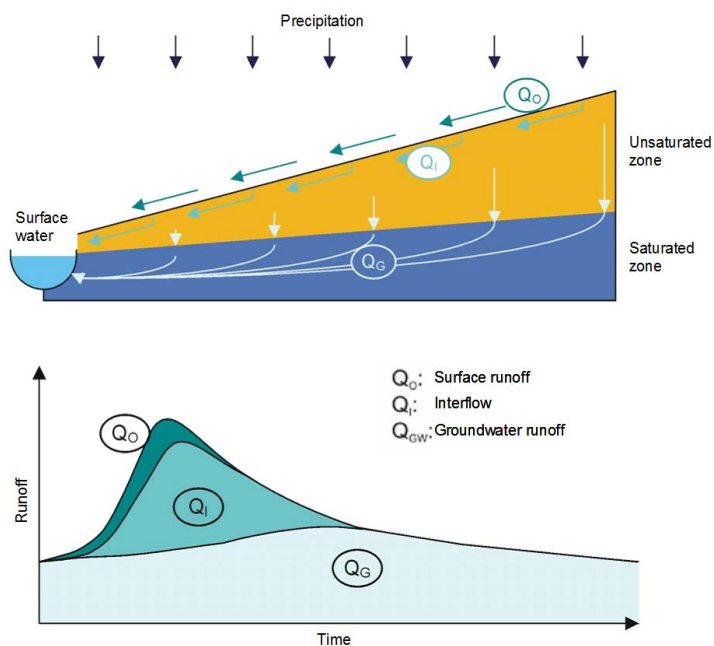
Figure 1-5: Runoff components according to Struckmeier (1997).
