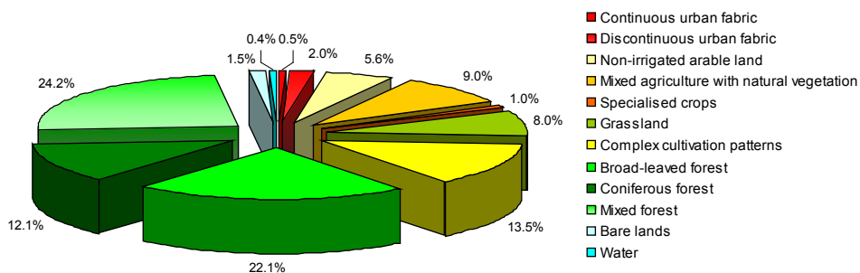
Figure 3-6: Percentages of area of the land cover units in Slovenia according to ATV-DVWK (2002).
