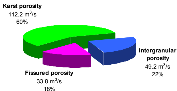
Figure 6-2: Distribution of groundwater recharge in Slovenia according to rock porosity type calculated by the GROWA-SI model.
