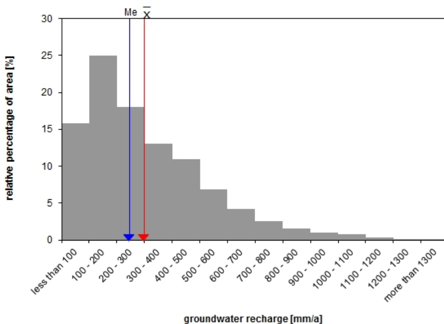
Figure 4-12: Frequency distribution of the calculated groundwater recharge in Slovenia.
